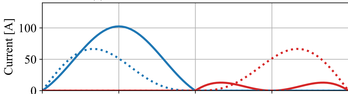
(a) Instantaneous IGBT and diode currents
