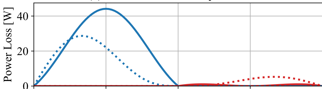
(b) Total IGBT and diode power losses
