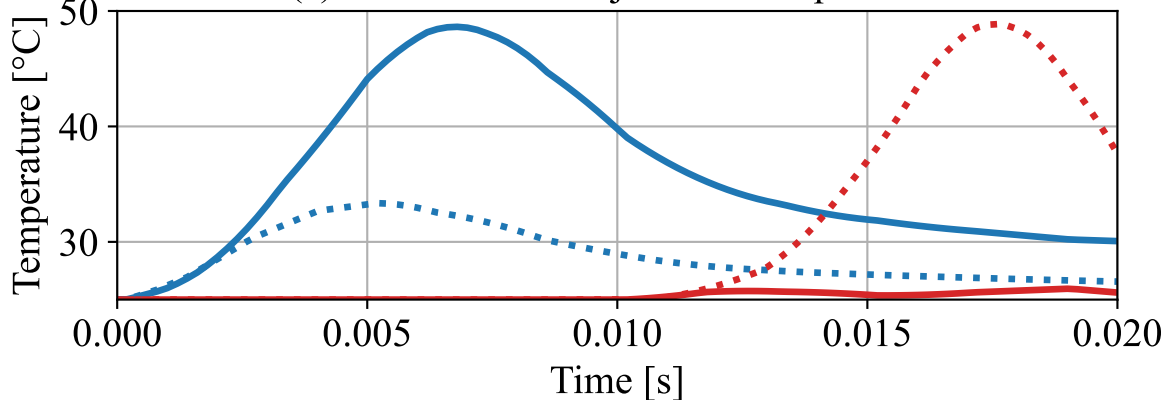
(c) IGBT and diode junction temperature
